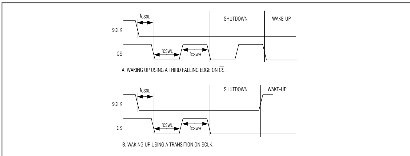
Figure 4. Shutdown Timing
